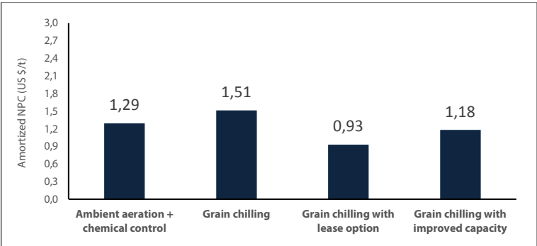
Fig. 6 Amortized Net Present Cost (NPC) of ambient aeration Strategy 4 and the grain chilling strategy with financial options for reducing the NPC.
