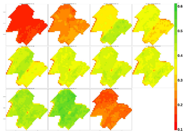
Fig. 1: Cloud-free NDVI 2016 images. High vigour vineyard.
