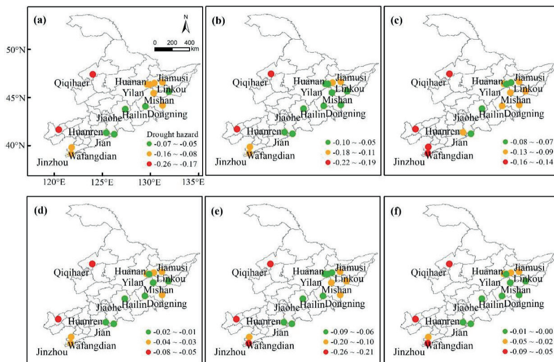
Fig. 3 Spatial distribution of drought hazard for different growth stages of grapevine in the Northeast wine region of China between 1981–2020 (a) bud burst; (b) shoot growth; (c) flowering; (d) berry development, (e) maturation; (f) full growth.
