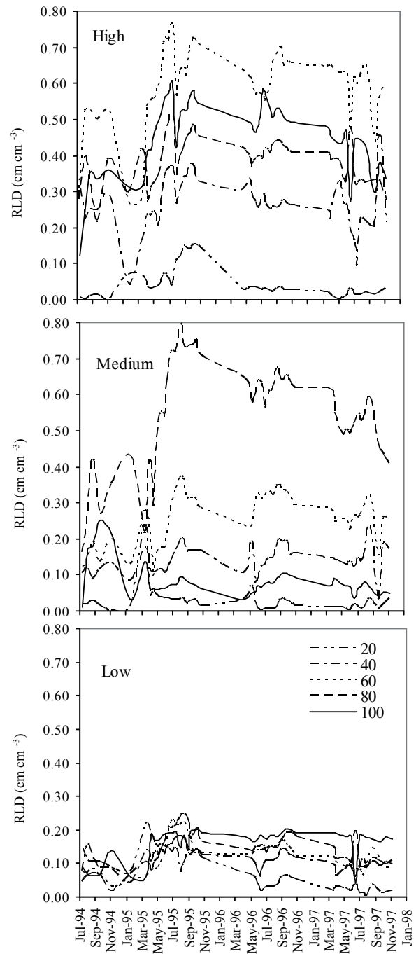
Fig. 4: Dynamic of root length density (RLD) in the soil depths from -20 cm to 80-100 cm for the vines of the groups High, Medium and Low.
